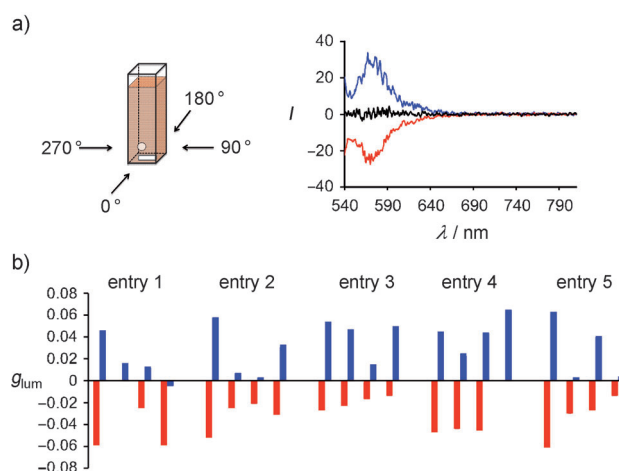
Figure 3. a) Circularly polarized luminescence (CPL) of the hydrogels of 2 ( 1.6 \times 10^{-5} \text{ M} ) in an aqueous solution of 1 (0.6 wt %) prepared with clockwise (CW, red) and counterclockwise (CCW, blue) stirring, and no stirring (black). For CPL spectroscopy, a beam of incoherent unpolarized incident light ( \varnothing = 5.0 \text{ mm} ) passed through the sample solution 3 mm above the center of the stir bar. b) To evaluate statistical distributions, multiple measurements of four different faces were employed. Statistical distributions of g_{\text{lum}} values in five different samples prepared by CW (red) and CCW (blue) operations in four faces of the sample cuvette. All original data are given in the Supporting Information.
